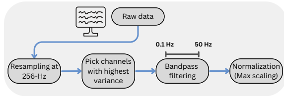
Fig. 2: Preprocessing pipeline.
