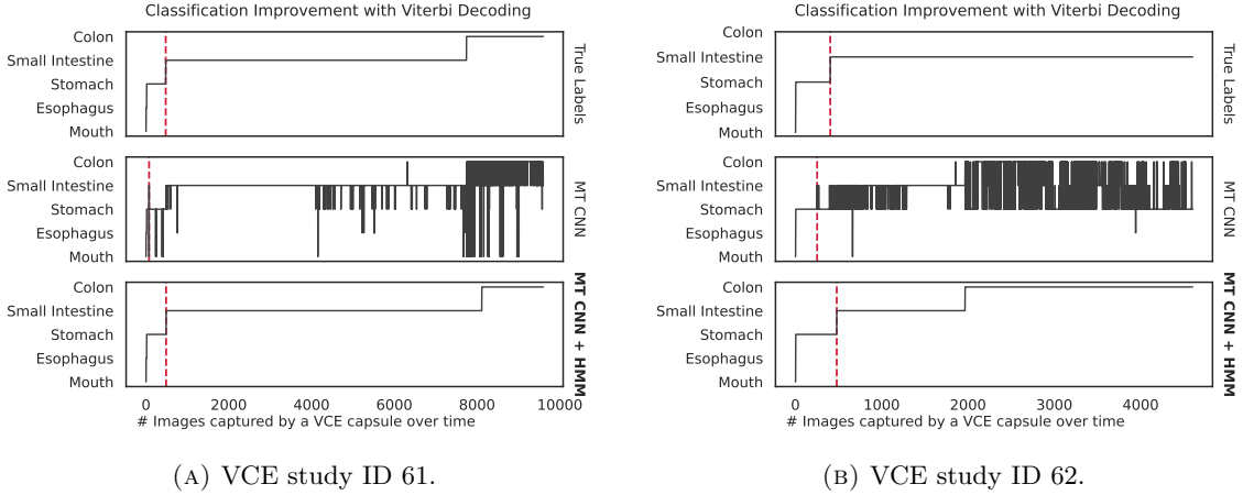
FIGURE 3.12: Classification performance of two single VCE studies shown for the multi-task CNN compared to the multi-task CNN in combination with the HMM using the DWA focal loss function.
