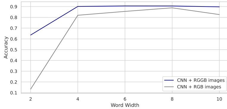
FIGURE 3.15: Accuracy of the hardware-suitable CNN tested on RGB and RGGB using different word widths (from A6 [Bau+25]).
