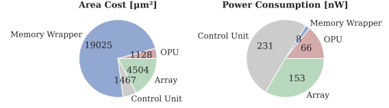
Fig. 7: Area costs and power consumption for different hardware components of the UltraTrail accelerator.
